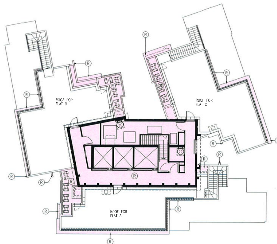
AQUA AVENUE TOWER 5 – ROOF FLOOR PLAN
