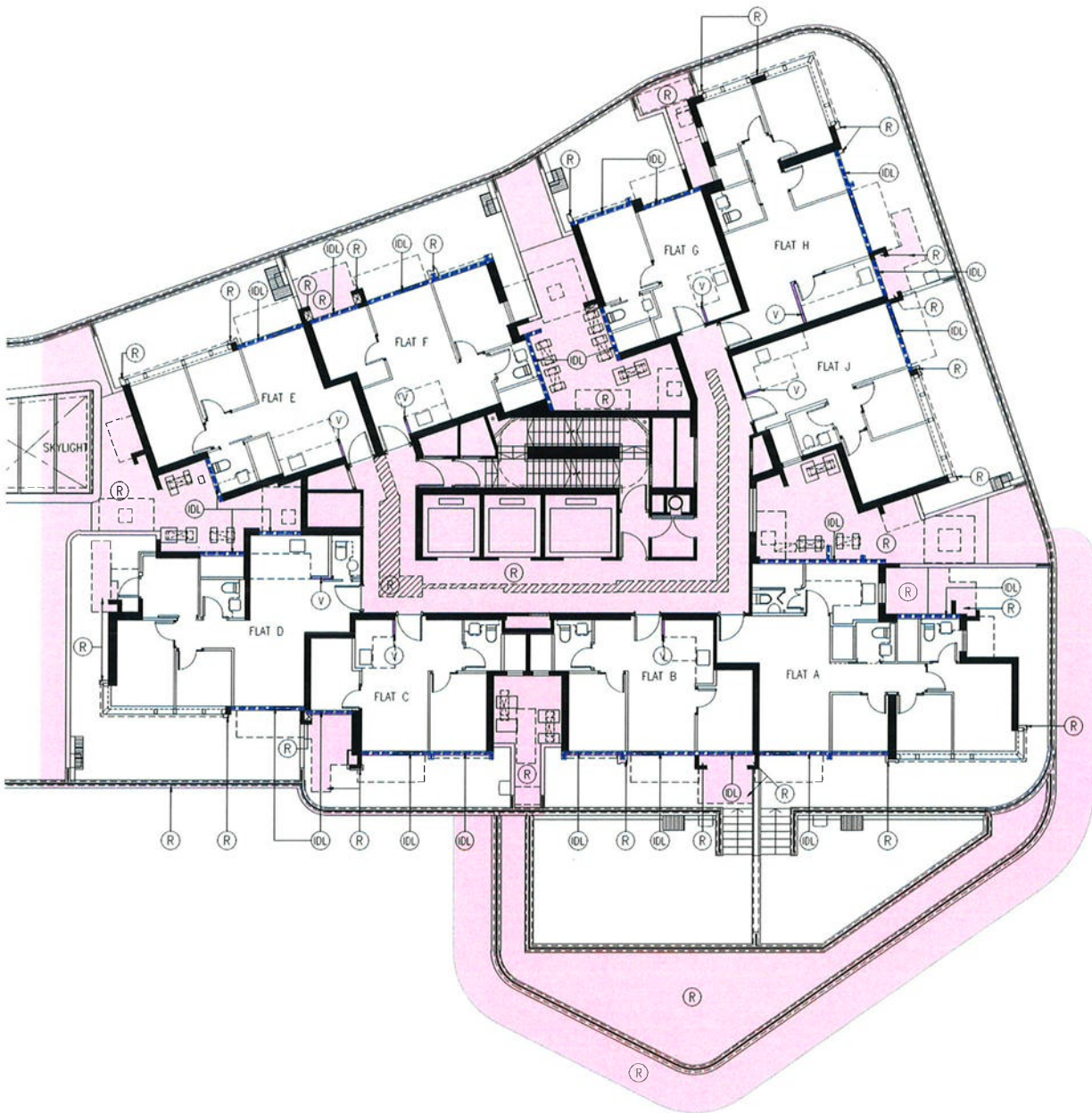
AQUA AVENUE TOWER 1 – 1ST FLOOR PLAN
