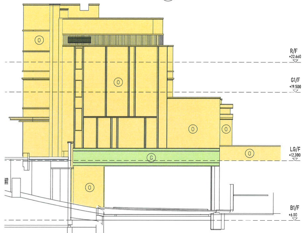
H ELEVATION H
